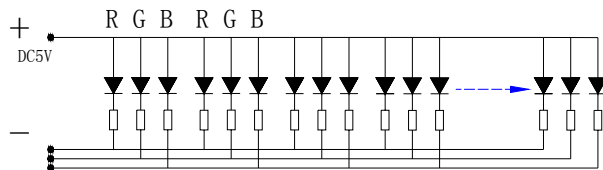
circuit for RGB color
