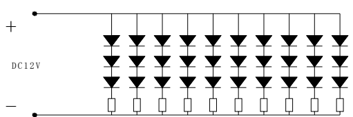
circuit for single color
